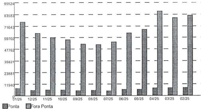
Consumo (kWh)
